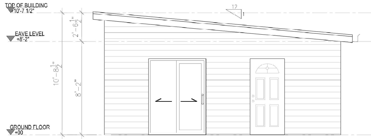
4 FRONT ELEVATION Scale 1"=1/4"
