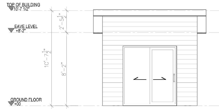
3 RIGHT SIDE ELEVATION Scale 1"=1/4"
