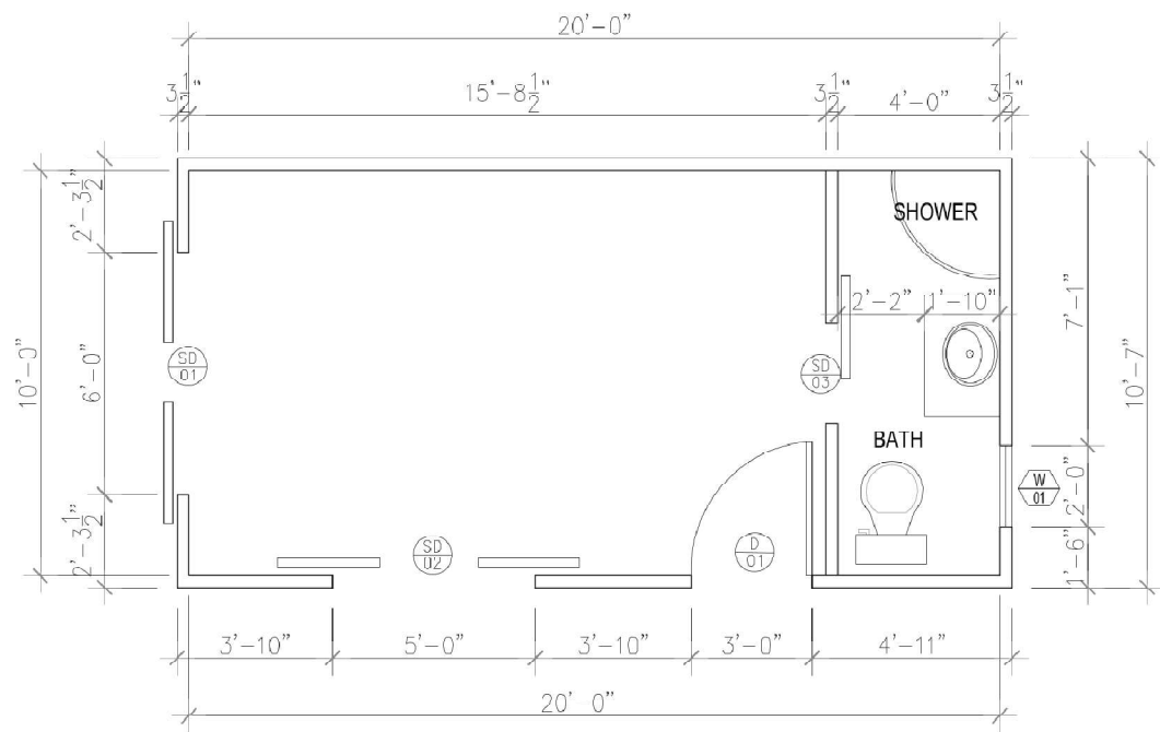
1 GROUND FLOOR PLAN Scale 1"=1/4"
