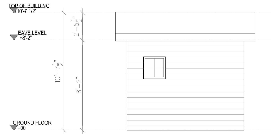
4 LEFT SIDE ELEVATION Scale 1"=1/4"
