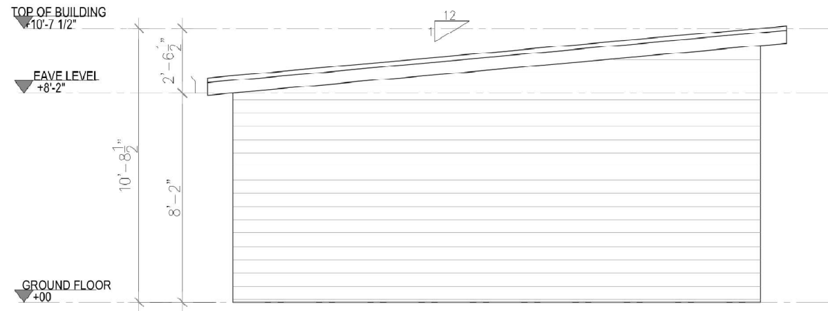
3 BACK ELEVATION Scale 1"=1/4"
