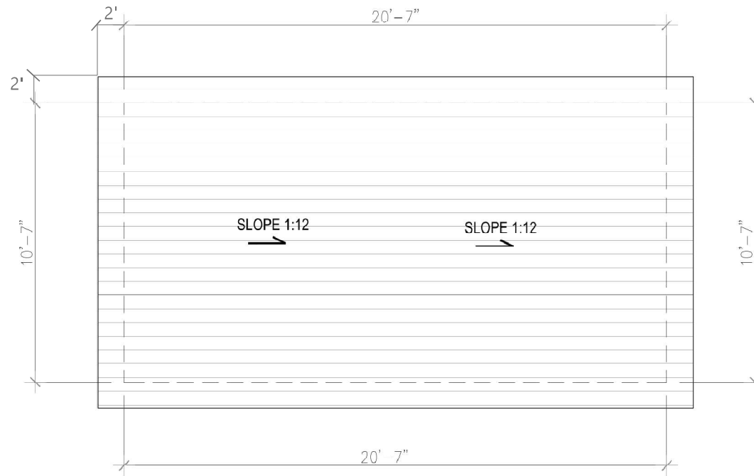
2 ROOF FLOOR PLAN Scale 1"=1/4"
