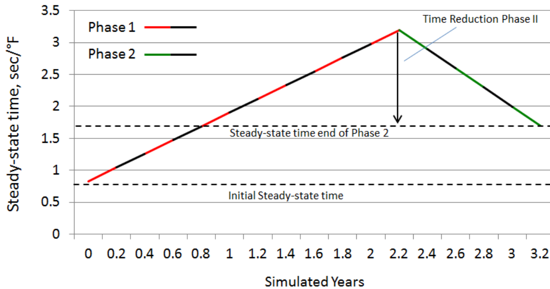
Figure 7. Phase II heaters displayed a decrease in time to steady state.
