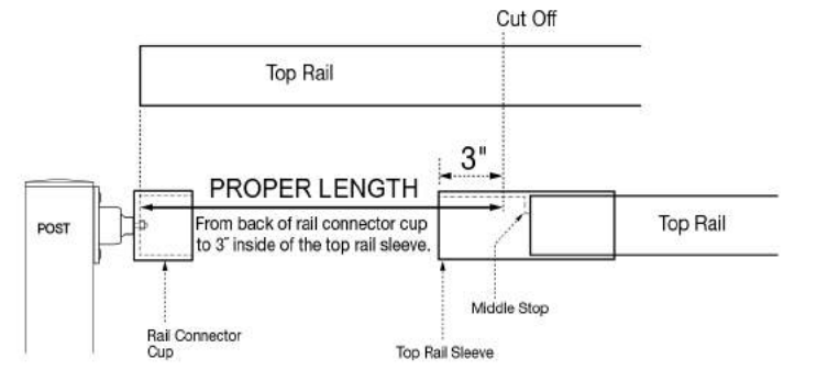
Fig. 11 Inserting the Terminating Top Rail
