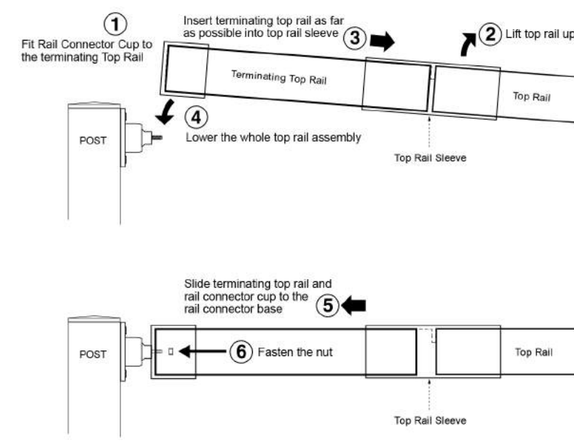
Fig. 11 Inserting the Terminating Top Rail
