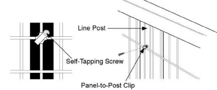
Fig. 18 Fence Panel Installation
