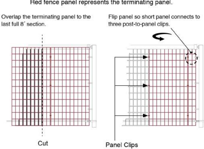
Fig. 17 Terminating Panel Installation
