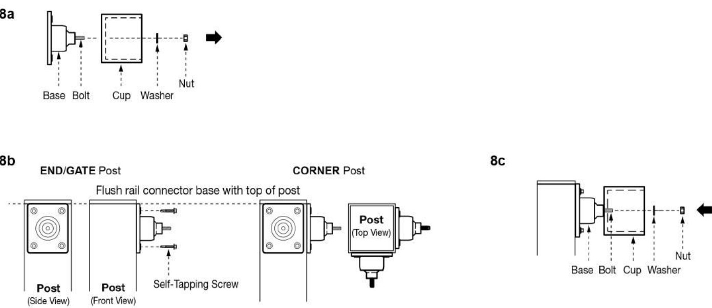
Fig. 8 Rail Connector Assembly
