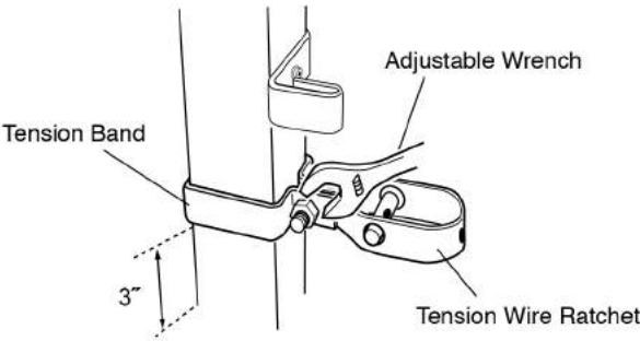
Fig. 12 Tension Band Installation
