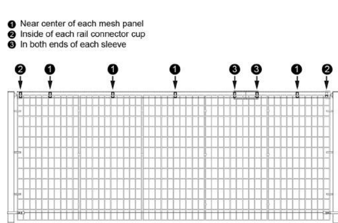
Fig. 16 Locations of Panel-to-Rail Clips and Panel Clips
