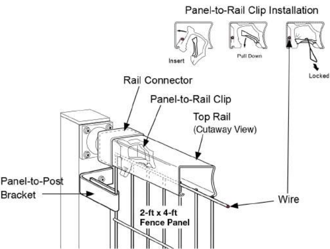
Fig. 15 Fence Panel Installation
