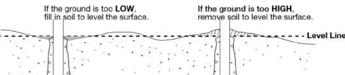
Fig. 3 Leveling Soil Surface for Adjusting Concrete Footings
