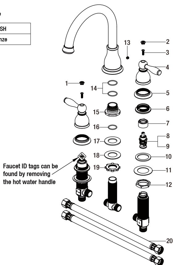
Mandouri 2-Handle Roman Tub Faucet in Bronze
