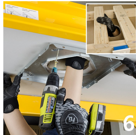
6 Using the included hardware, secure the ceiling plate into the wooden support created earlier. Ensure the screws are fastened into the 2x4s.
