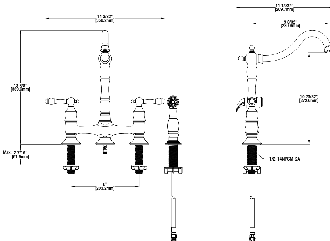
INSTALLATION DIMENSIONS
