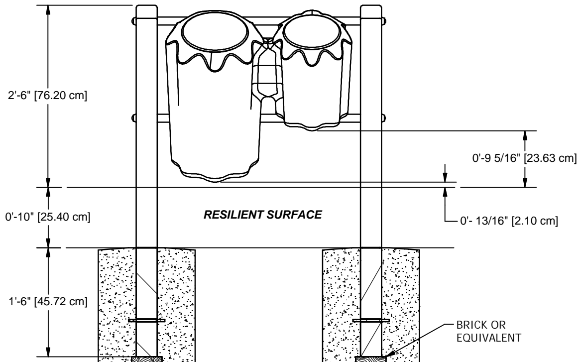
ELEVATION VIEW
