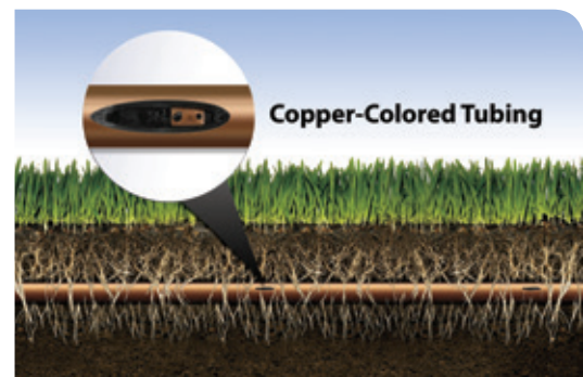
XFS Sub-Surface Dripline with Copper Shield™ Technology
