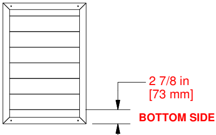
WP04 WALL PANEL - W2A03784 (x2) 1"x16 7/8"x24 5/8" (24x430x627)
