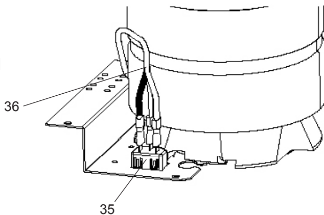
Fig. 12 220V/240V Detail
