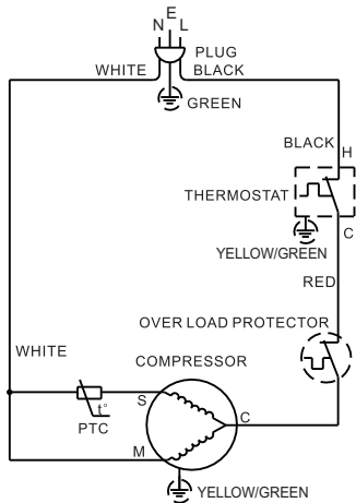
CIRCUIT DIAGRAM
