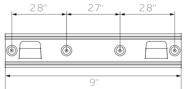
LOWER BRACKET
