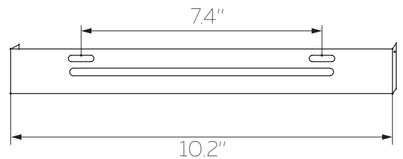
UPPER BRACKET
