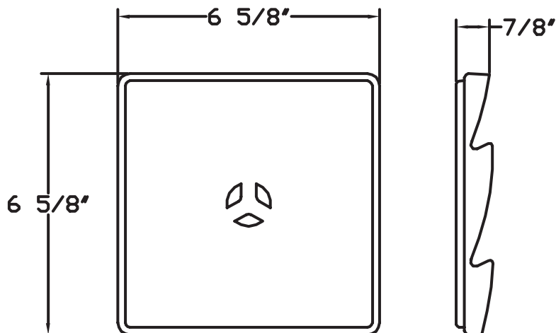
SURFACE MOUNT FOR TRIPLE 3" SIDING
