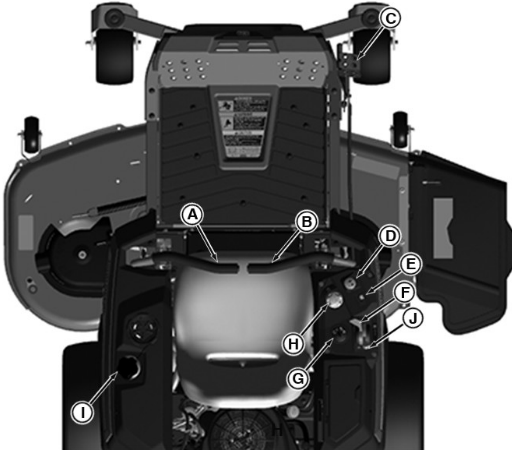
Operator's Station Controls for Model Z330R
