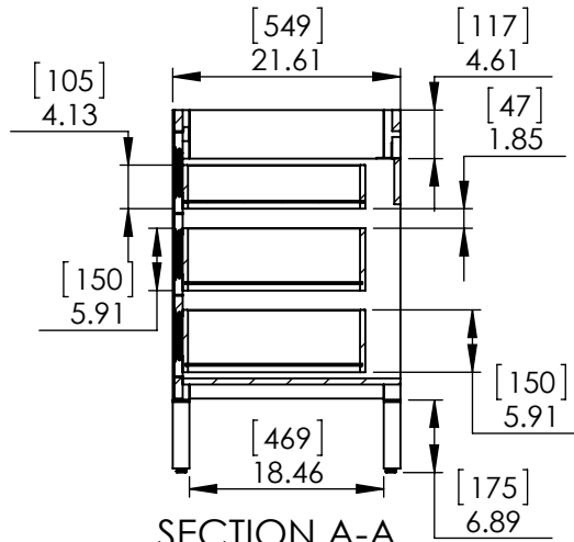
SECTION A-A Side View
