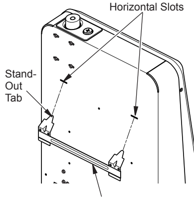
Figure 9 - Mounting Heater Onto Mounting Bracket
