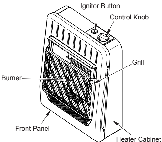
Figure 1 - Vent-Free Gas Heater
