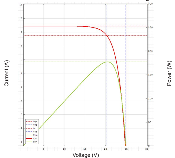
RNG-175DB-H Characteristics Versus Voltage
