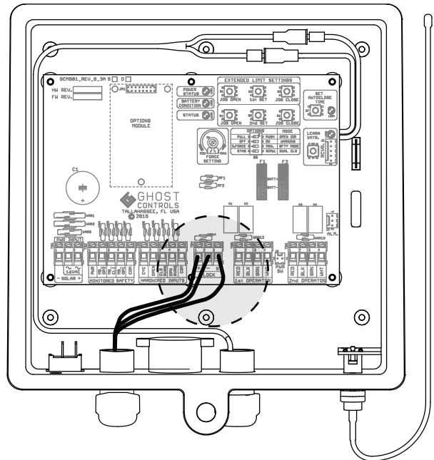
Control Box
