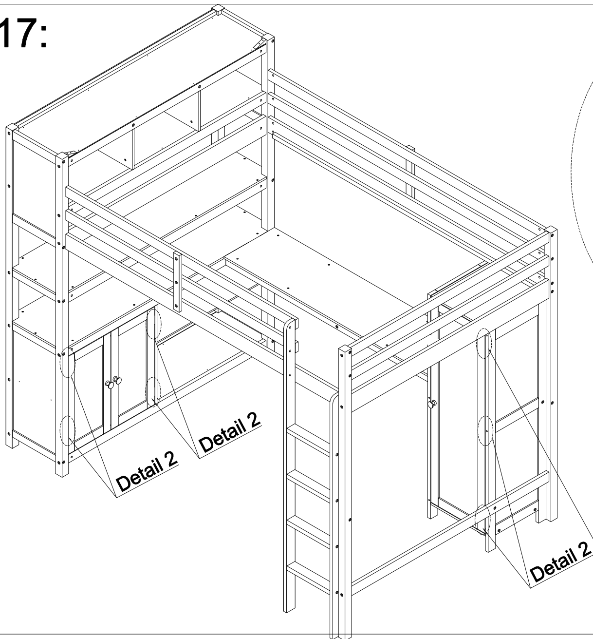
Detail 2(x7)
