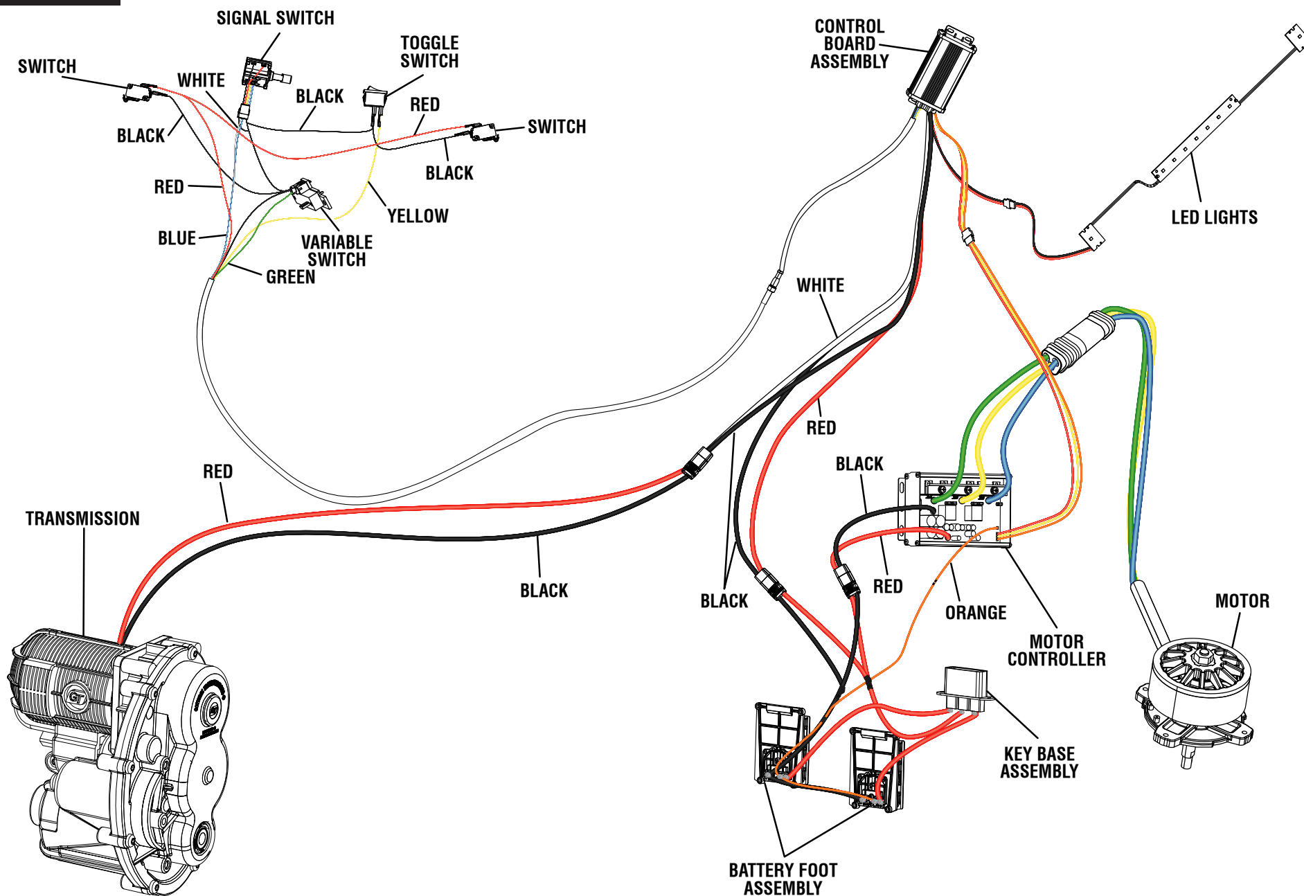
WIRING DIAGRAM
