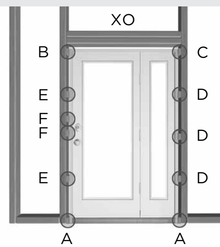
FIGURE 18: Install shims in the correct location and in the correct sequence.
