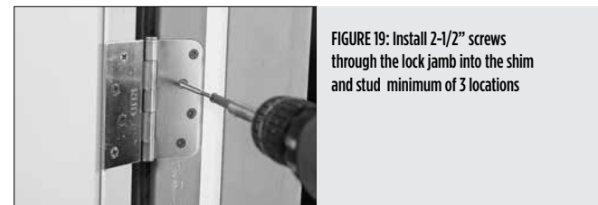
FIGURE 19: Install 2-1/2" screws through the lock jamb into the shim and stud. Minimum of 3 locations.
