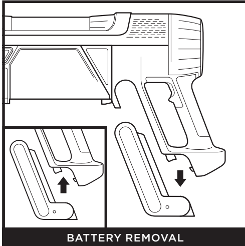
BATTERY REMOVAL
