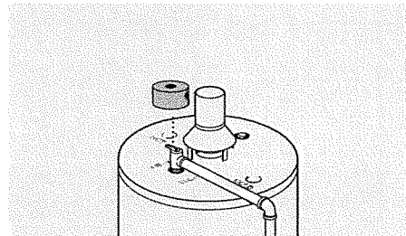
Typical Top Connect T & P Arrangement.
