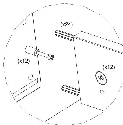
Detail F
