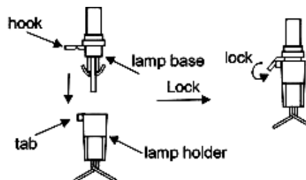
Fig. 2 Replace with the spare lamp
