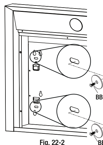
FRAMED CABINET
