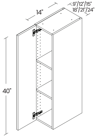
40" HIGH 1 DOOR
