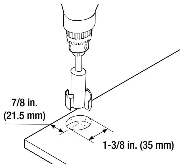
Diagram for Drilling Hinge Cup
