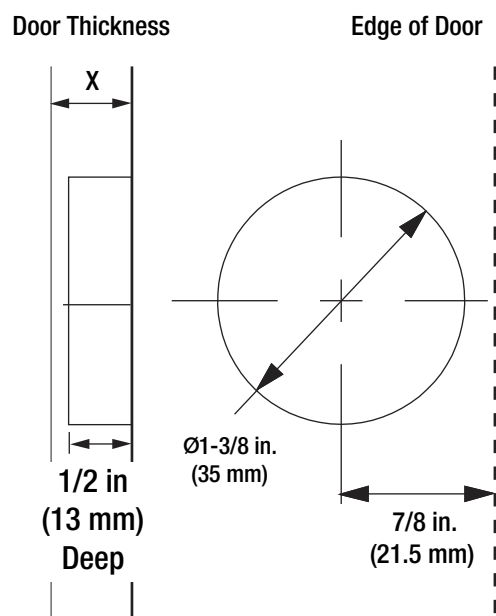
Diagram for Drilling Hinge Cup
